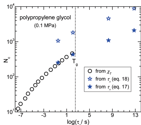
Figure 6. Number of dynamically correlated PPG repeat units determined from \chi_T (open circles) at various temperatures and from \tau_x (solid stars: eq 17; open stars: eq 18) at four temperatures (corresponding to the respective T_g for four molecular weights). Dielectric data are from ref 13.
